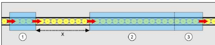
In case of particularly dirty cylinders a soap application section can be installed (1) before the washing section. The X distance depends on the time necessary for the soap mixture to dissolve the dirt on the cylinders before rinsing in the washing section (2).
